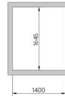
Shaft plan view
